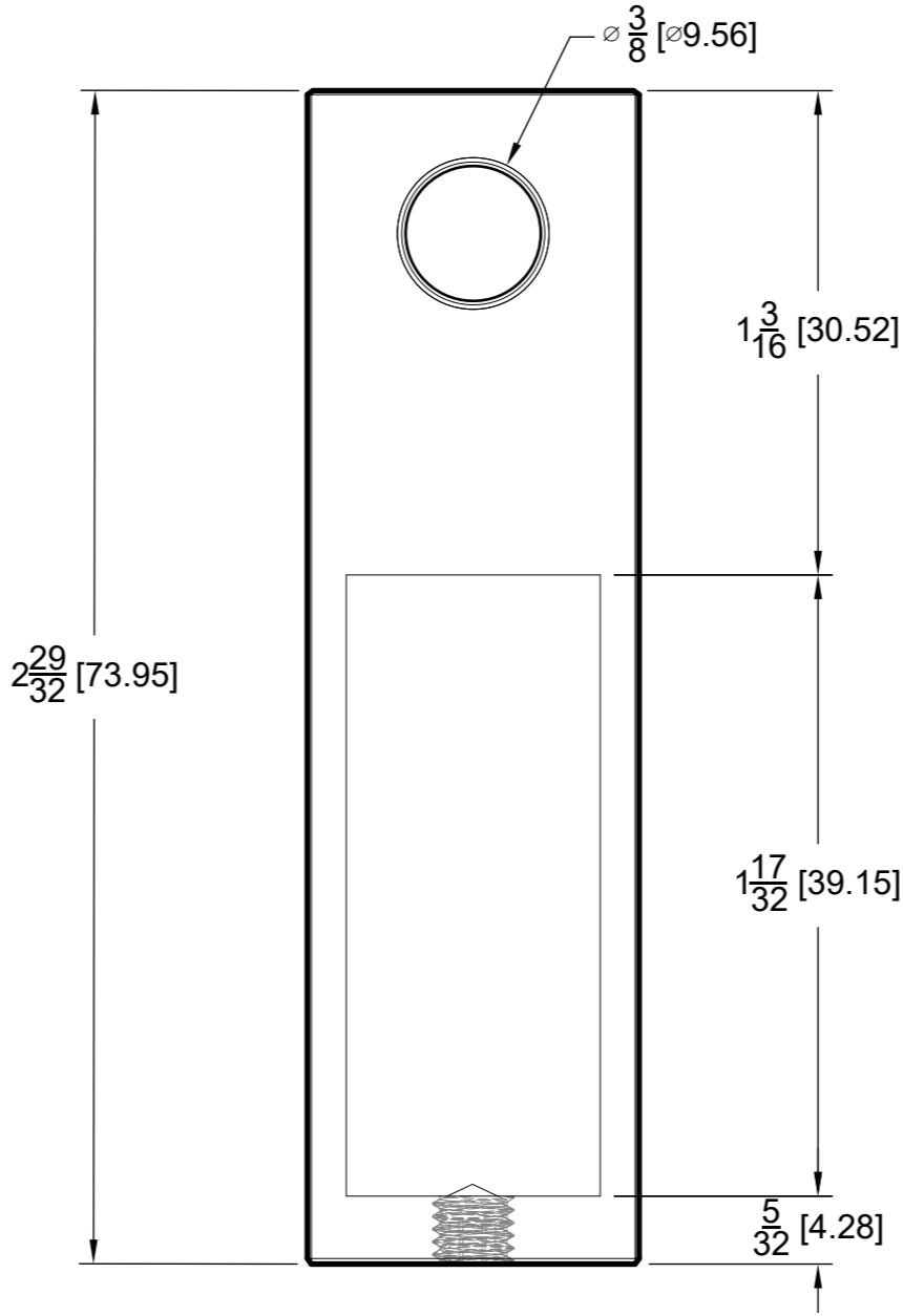
FRONT VIEW
