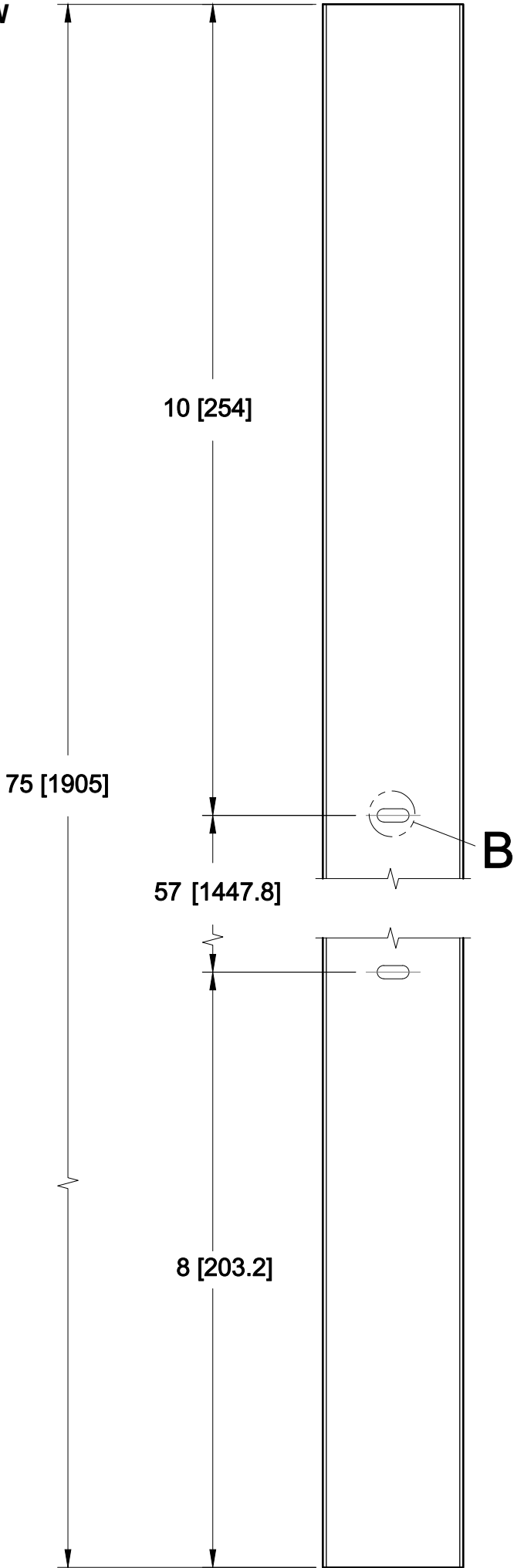
SIDE VIEW
