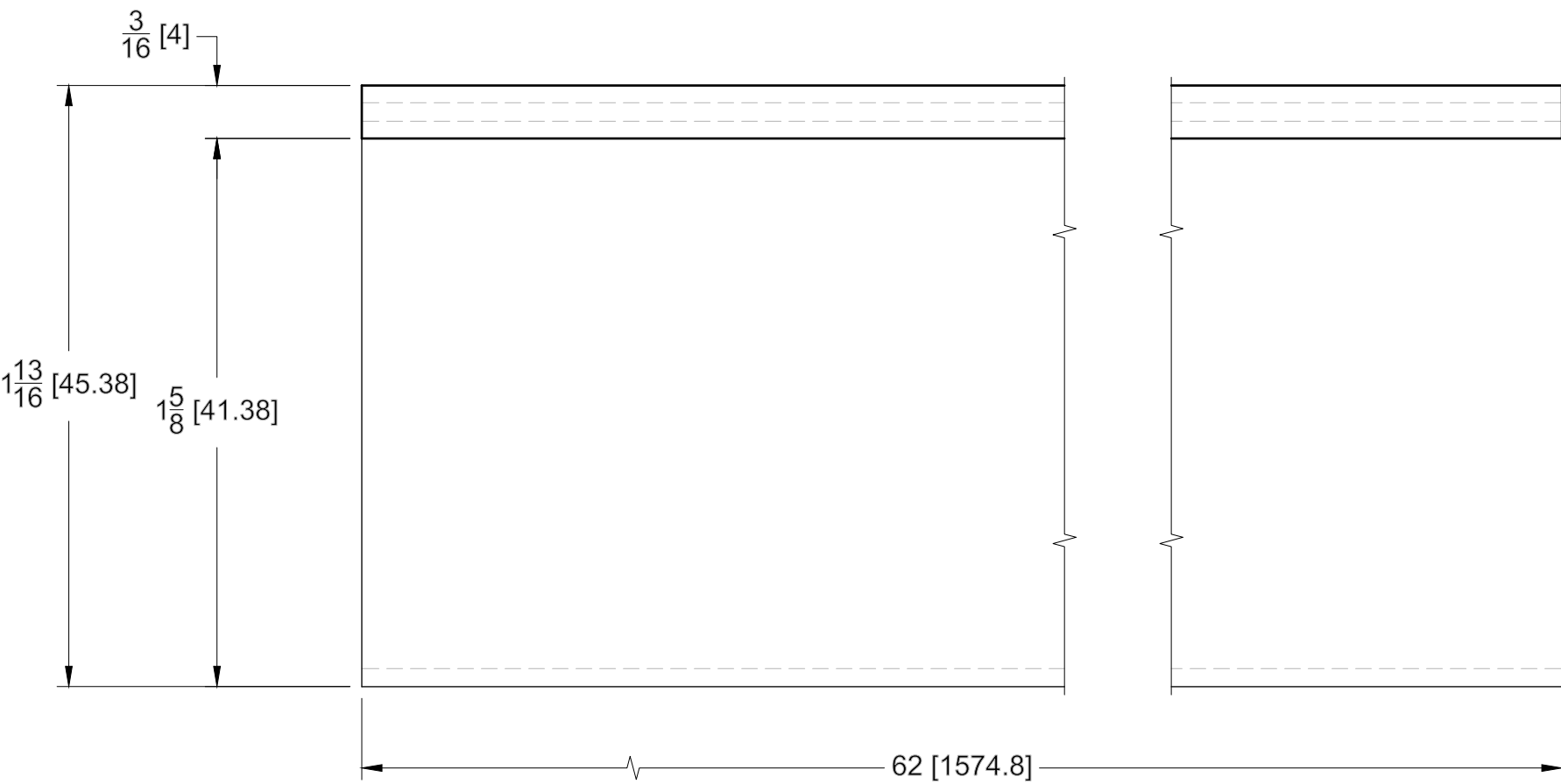
TOP VIEW
