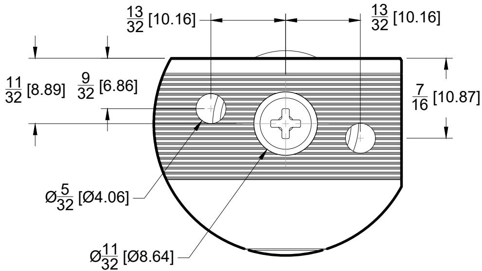
DETAIL A
