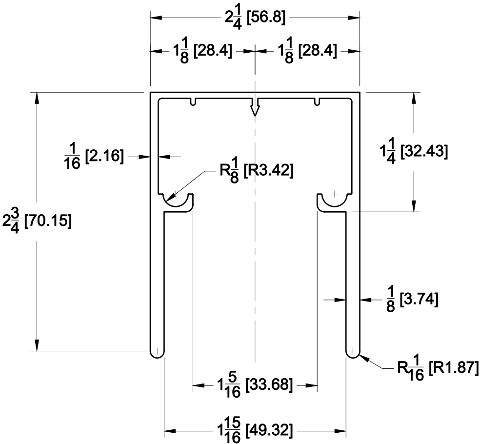
SIDE VIEW
