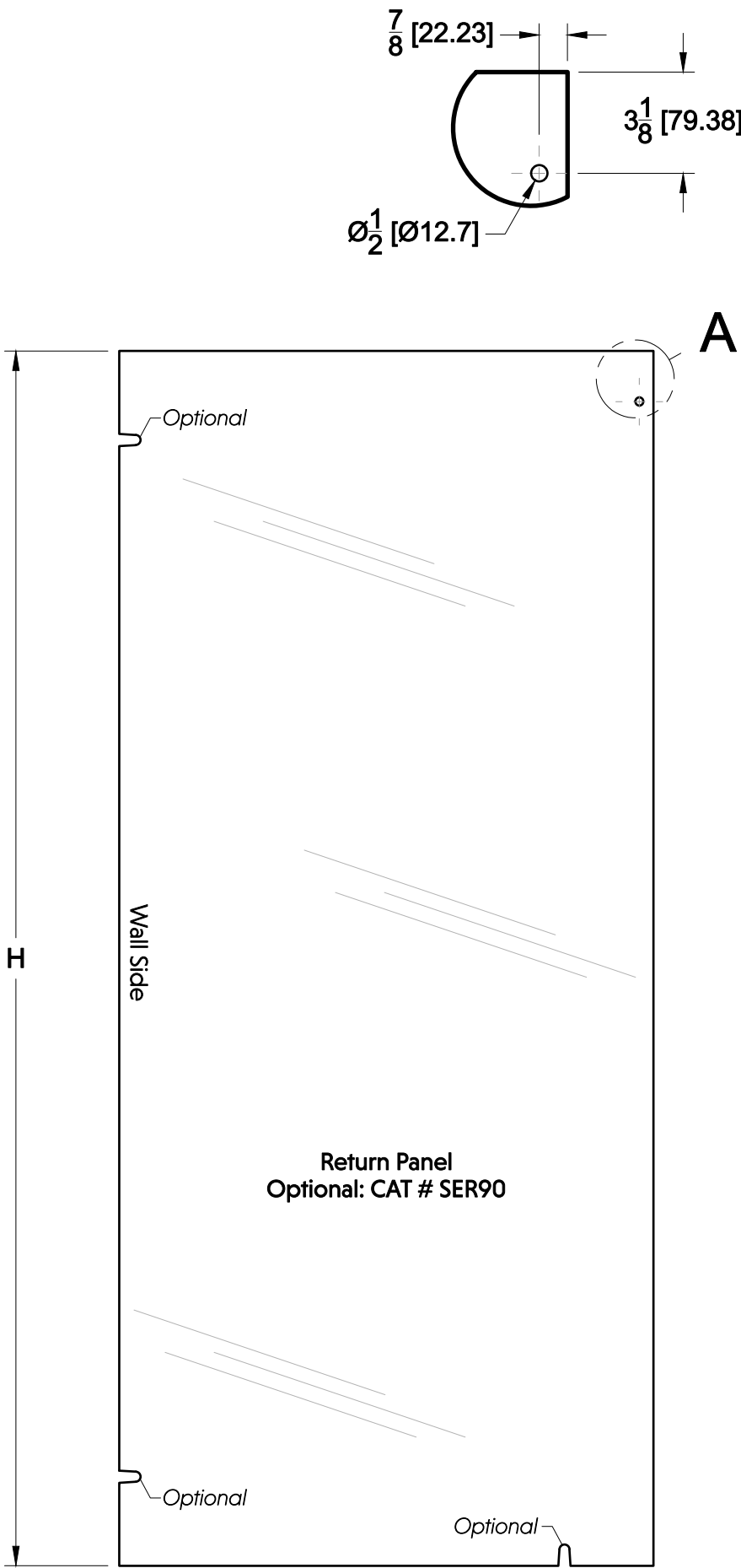
DETAIL A
