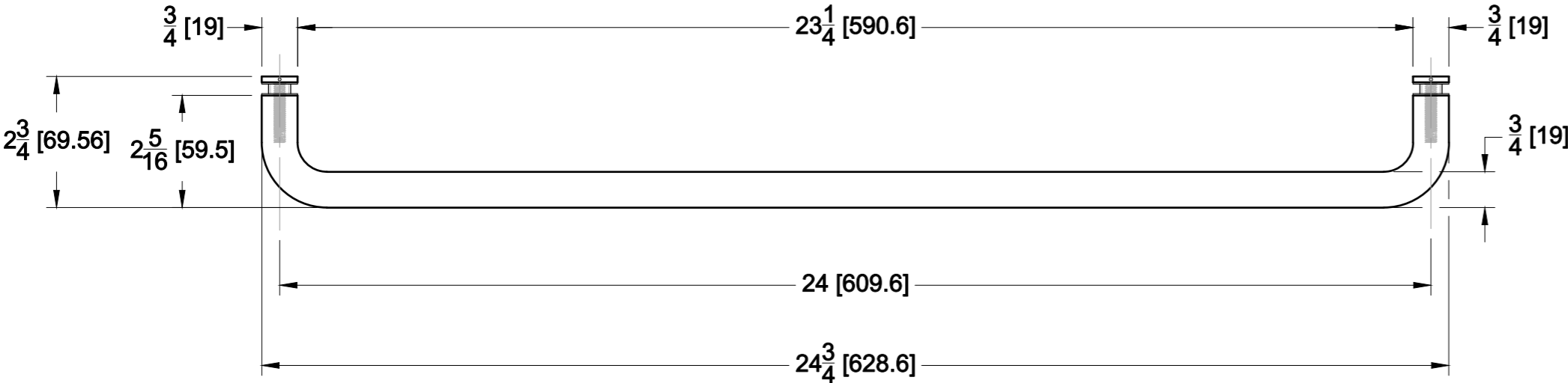
FRONT VIEW
