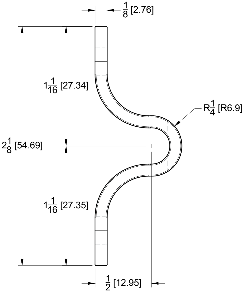
TOP VIEW
