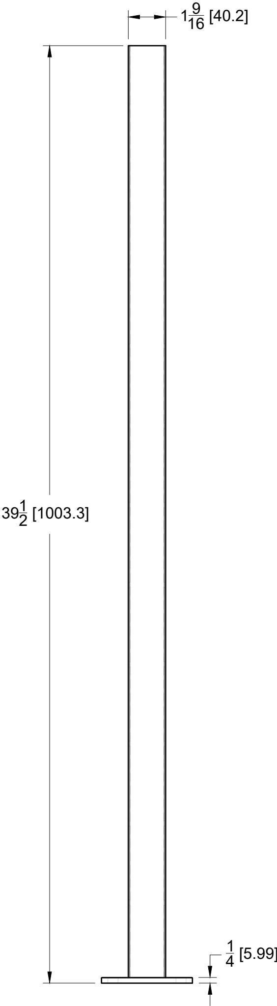
SIDE VIEW
