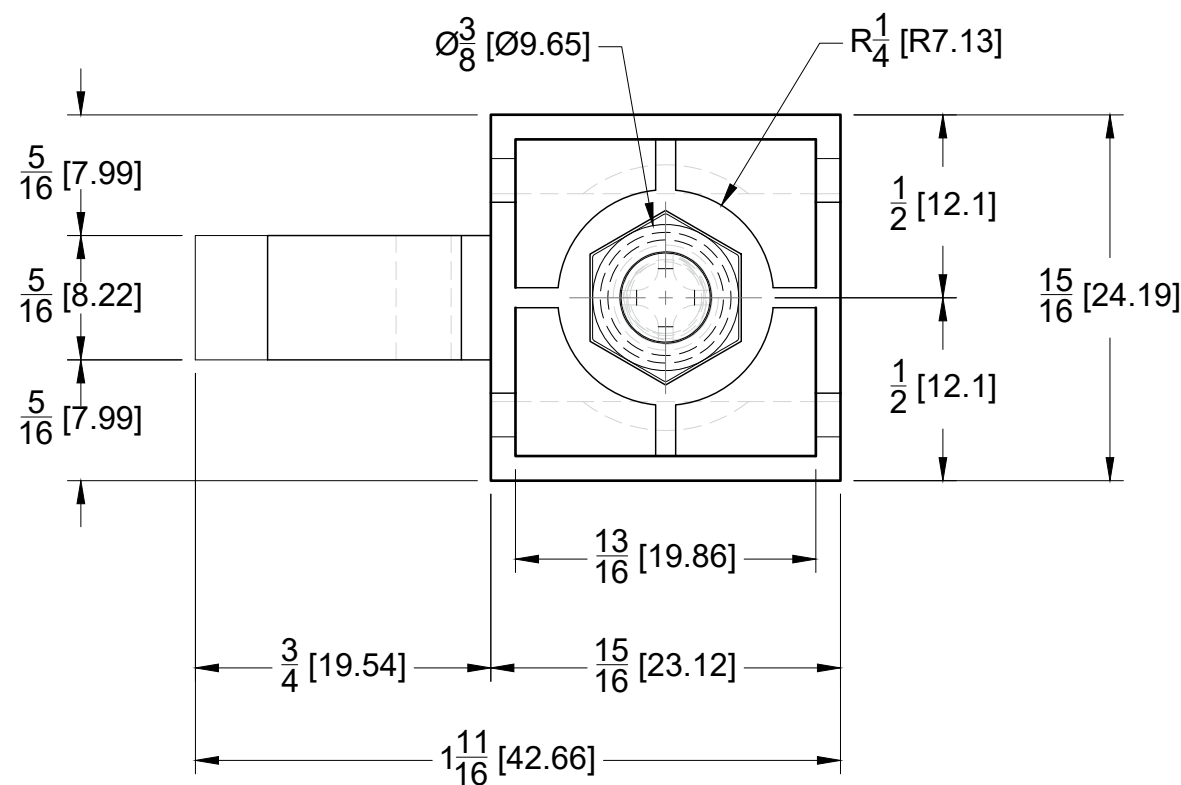
TOP VIEW
