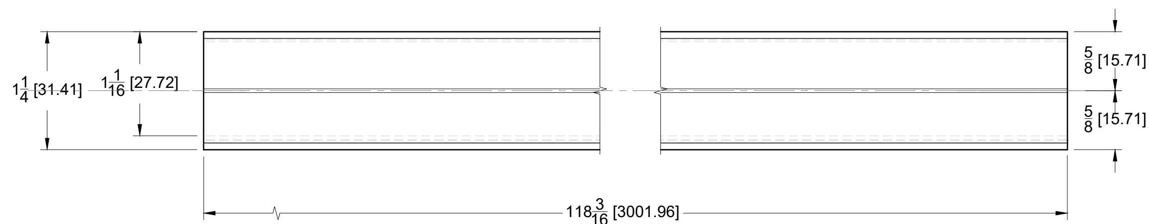
FRONT VIEW
