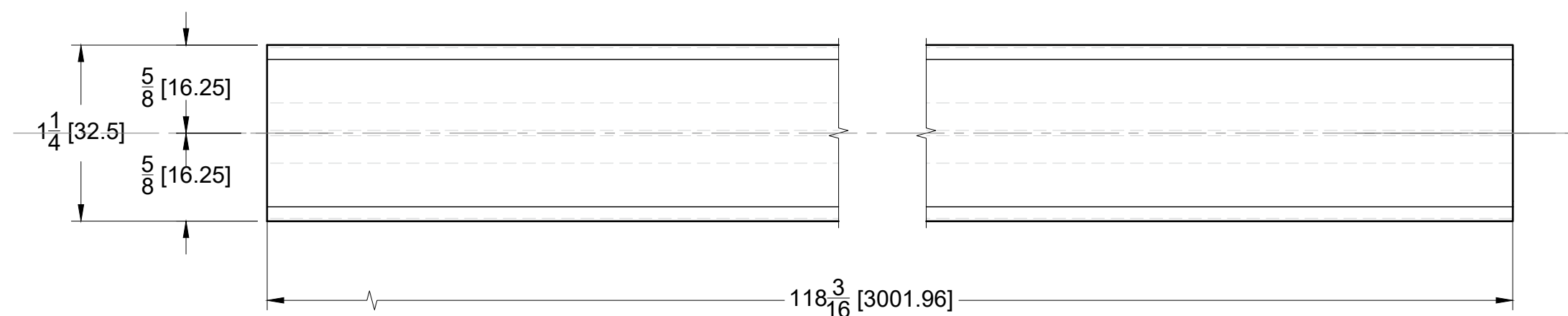
TOP VIEW
