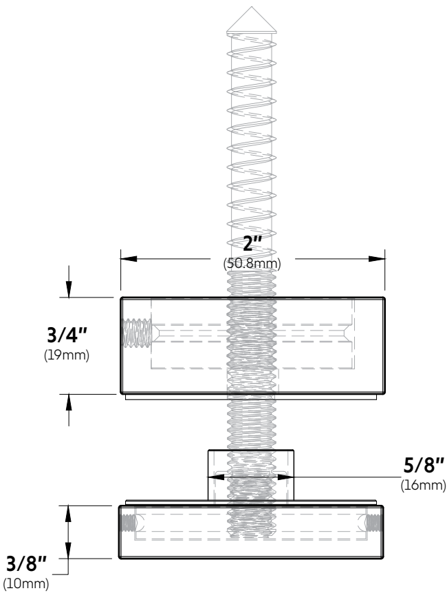
TOP VIEW
