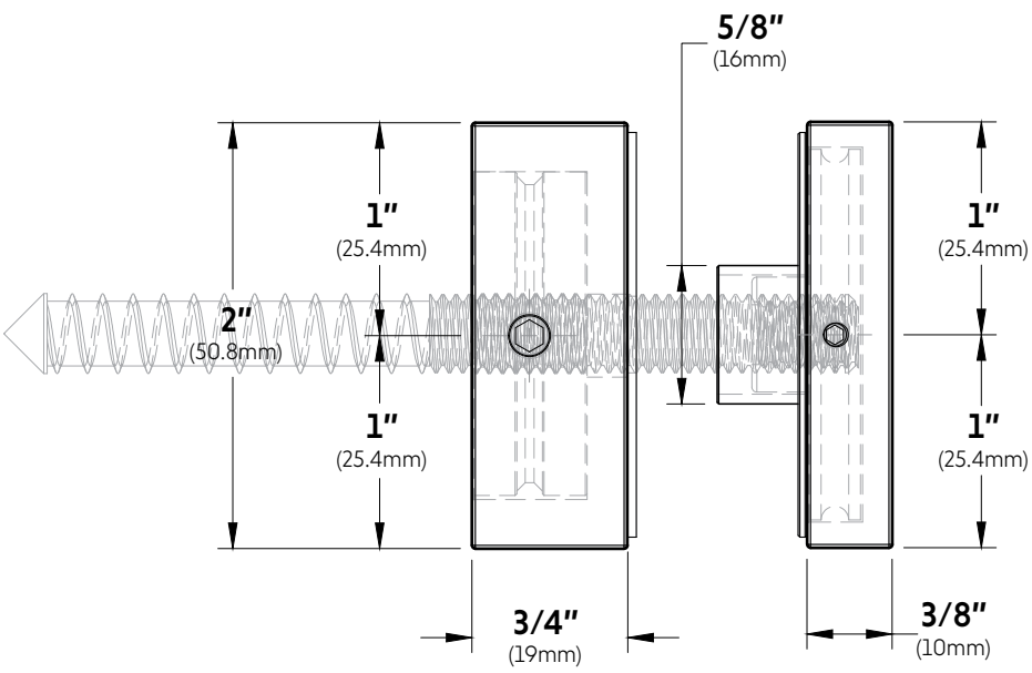
SIDE VIEW
