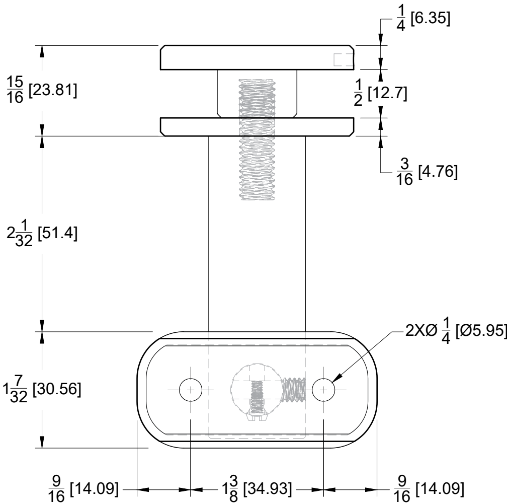
TOP VIEW
