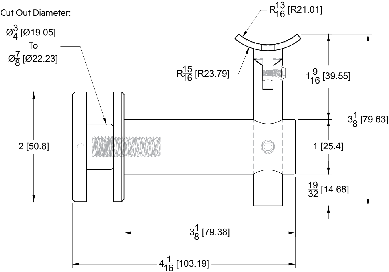
SIDE VIEW
