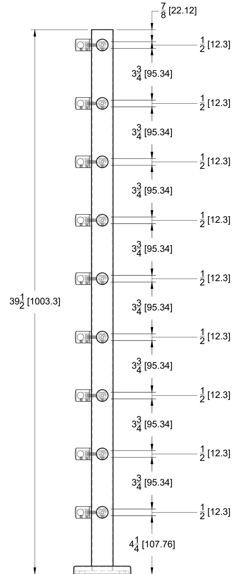
SIDE VIEW
