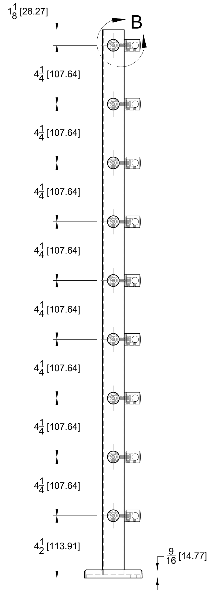
FRONT VIEW
