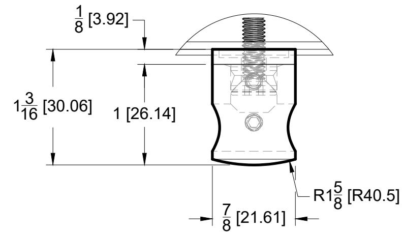
DETAIL B
