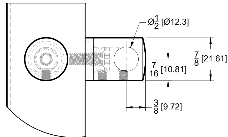
DETAIL B
