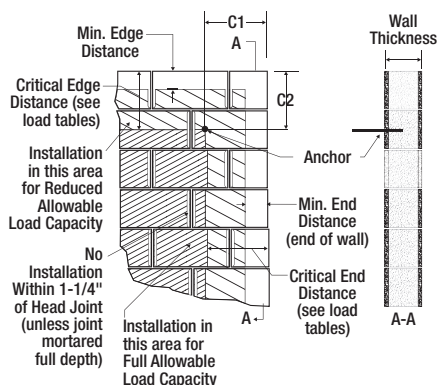
Illustration of Screw-Bolt+ Anchors Installed into Grouted Concrete Masonry Wall
