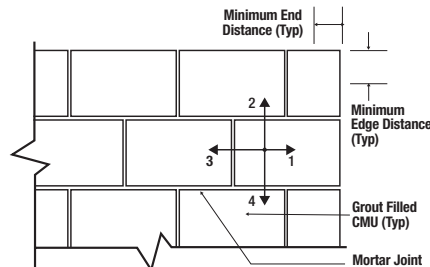
Direction of Shear Loading in Relation to Edge and End of Masonry Wall
