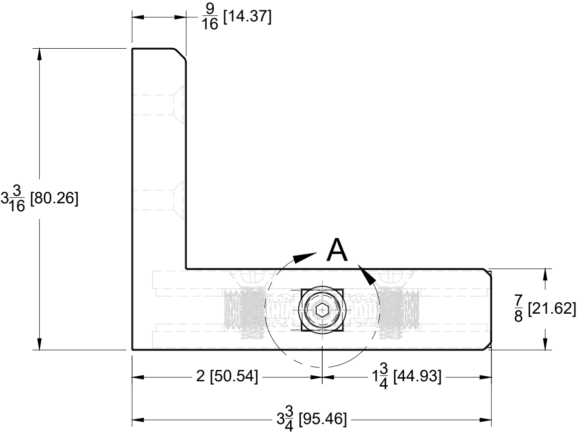
TOP VIEW
